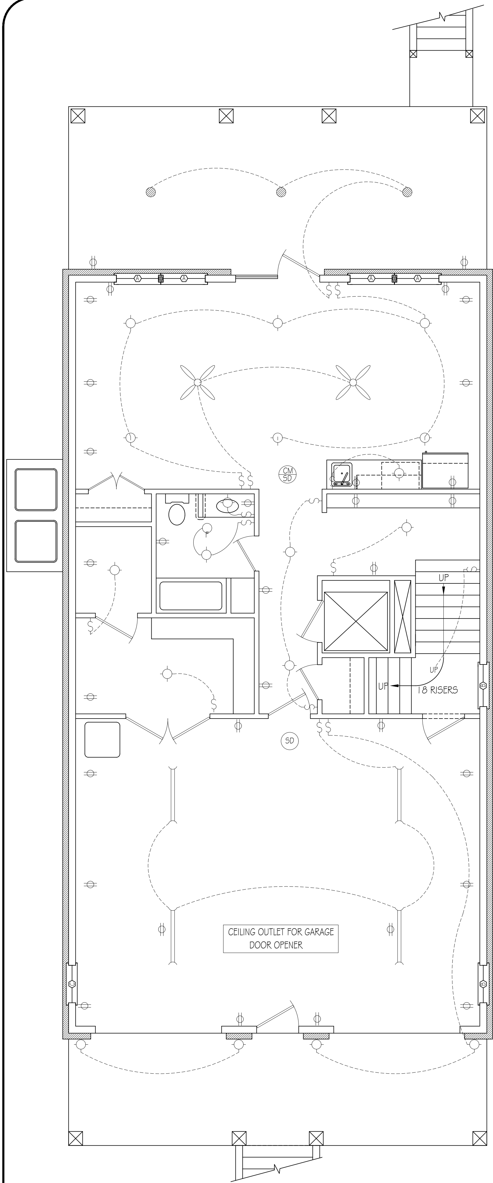
GROUND LEVEL ELECTRICAL 9'-0" CEILING HEIGHT SCALE: 1/4"=1'-0"
