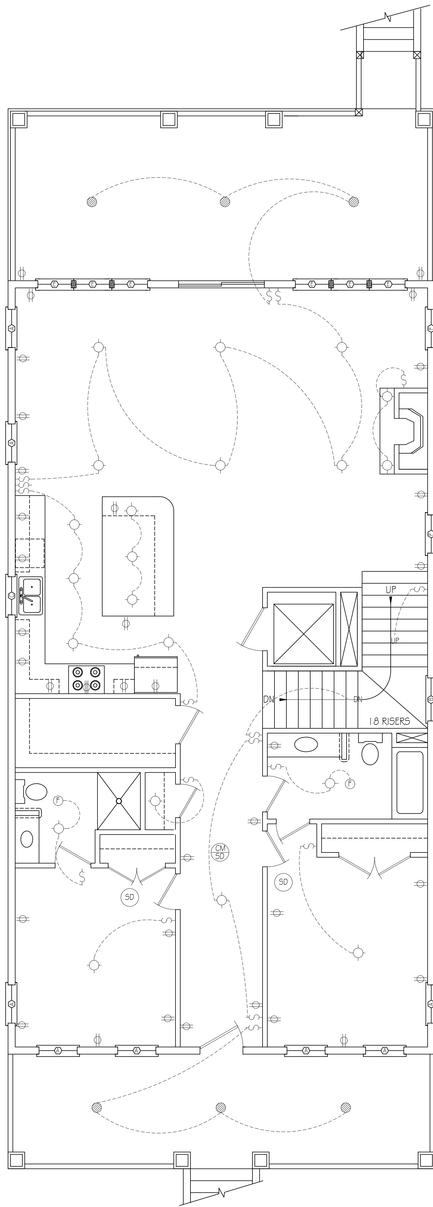
FIRST FLOOR ELECTRICAL 10'-0" CEILING HEIGHT SCALE: 1/4"=1'-0"
