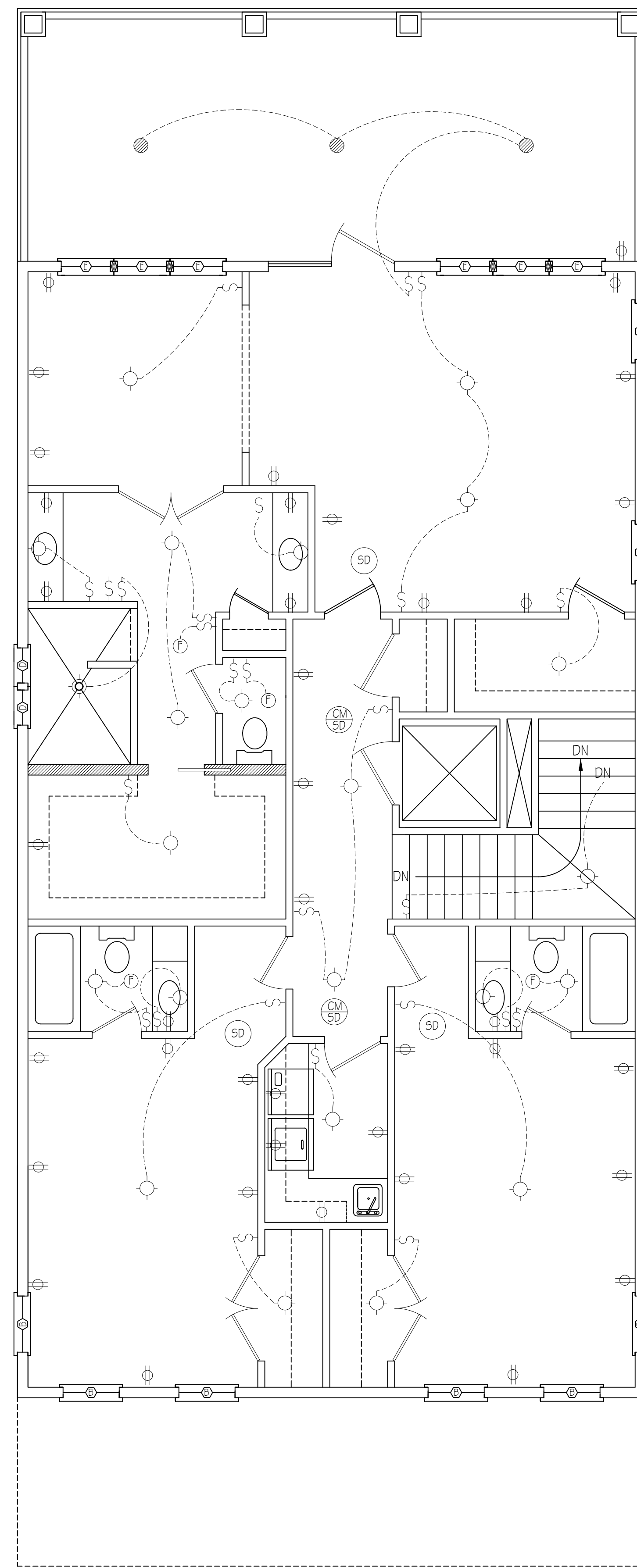
SECOND FLOOR ELECTRICAL 9'-0" CEILING HEIGHT SCALE: 1/4"=1'-0"
